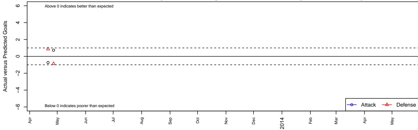
WUSC Boca Jrs. B00 Dots are actual minus expected GF (blue circles) and GA (red triangles). Blue line is smoothed change in attack strength. Red is smoothed change in defense strength.
